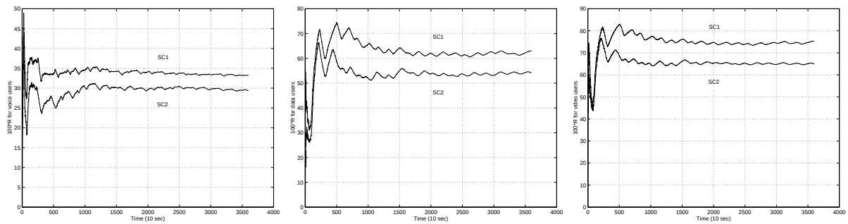
Figure 11. Percentage of refused voice, data and video calls
