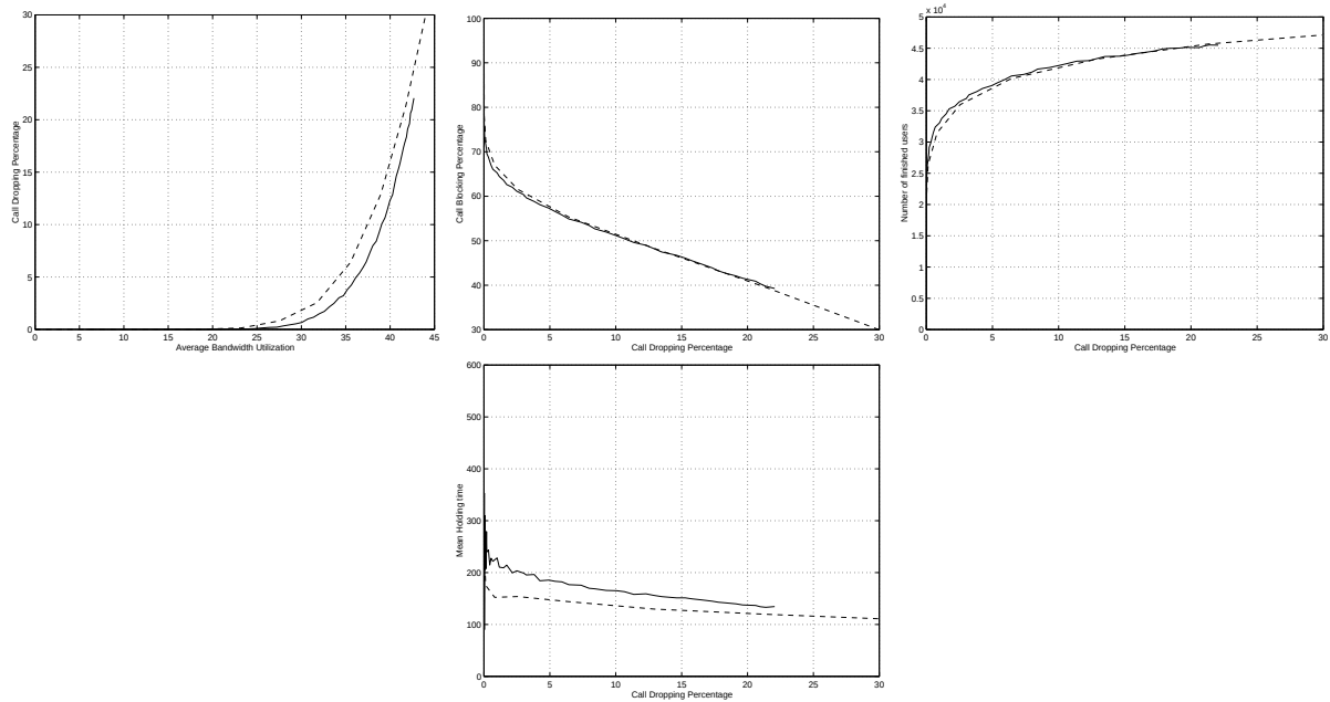
Figure 5. (5.a, 5.b, 5.c and 5.d) Comparing the two schemes (data traffic only)
