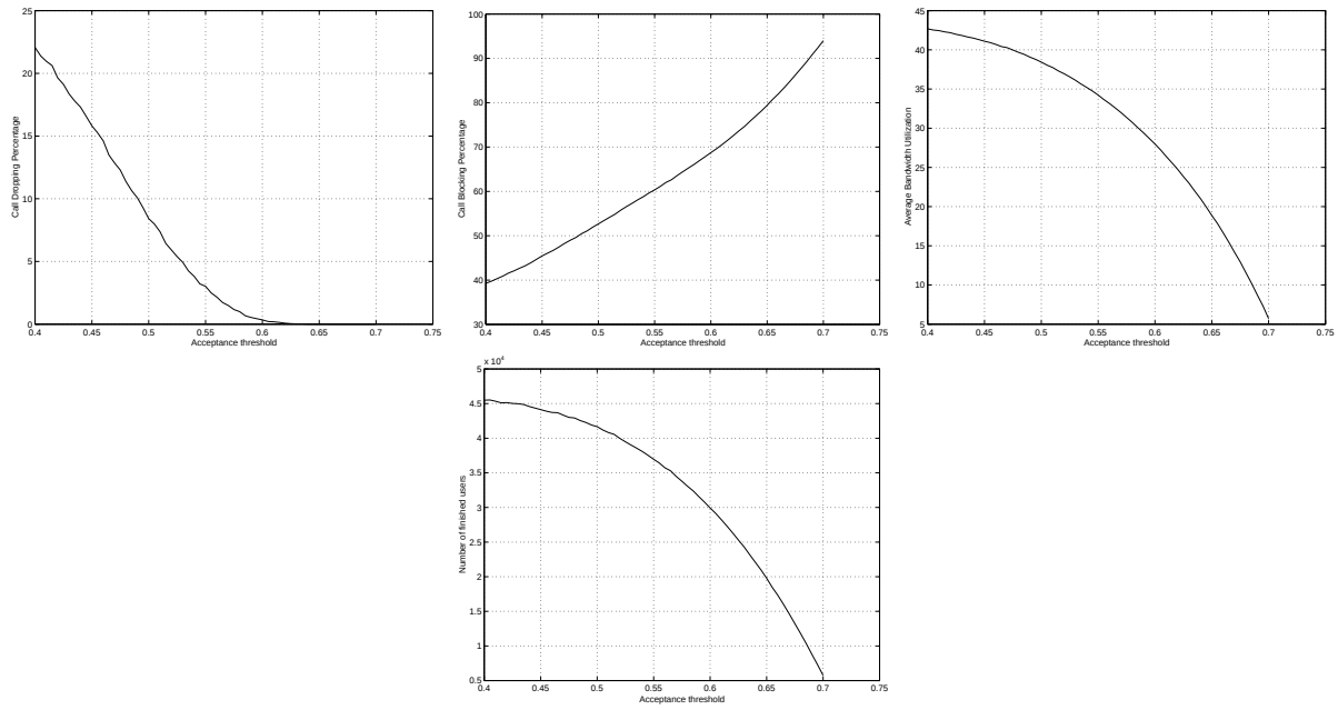
Figure 4. (4.a, 4.b, 4.c and 4.d) Simulation results for DCAC according to the acceptance threshold
